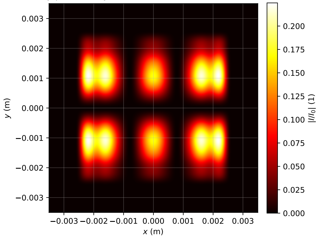
Intensity profile I(x, y, z = 3.981)/I_0 , P_{in}=0.5P_{cr} , artificial time
